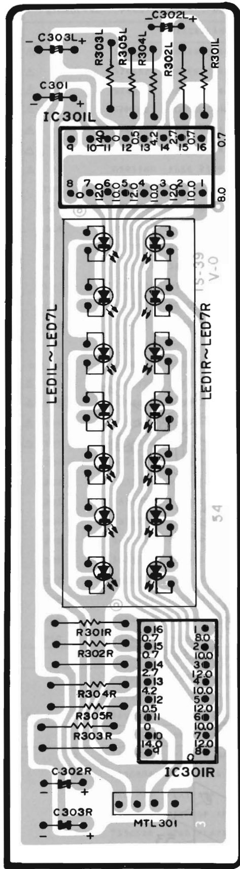
LED METER
